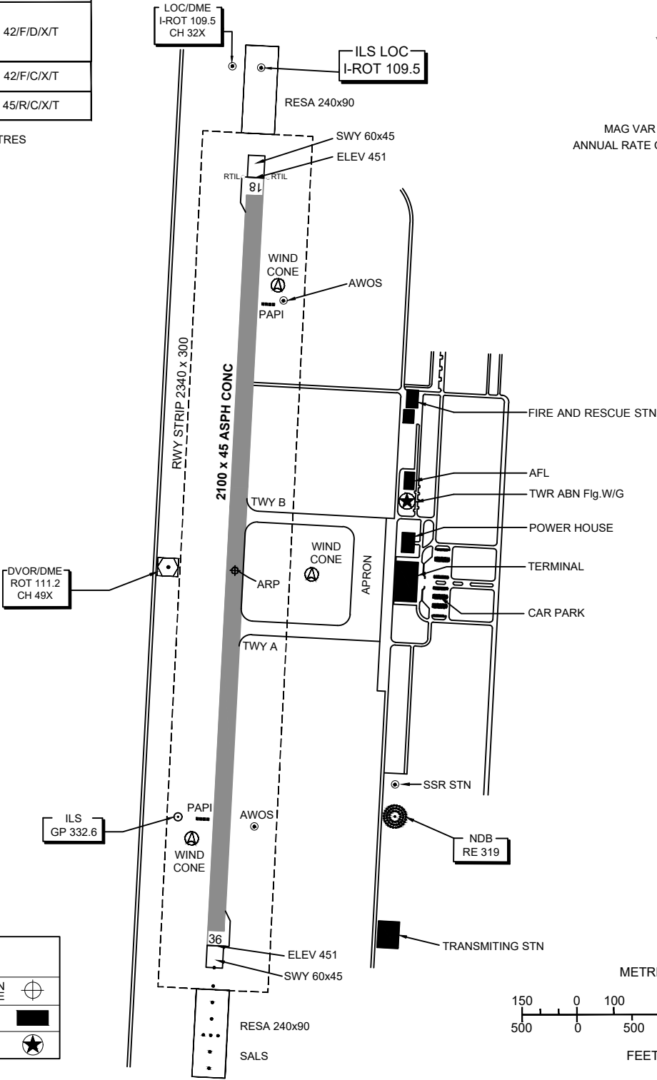
MARKING AIDS RWY 18/36 AND EXIT TWY
