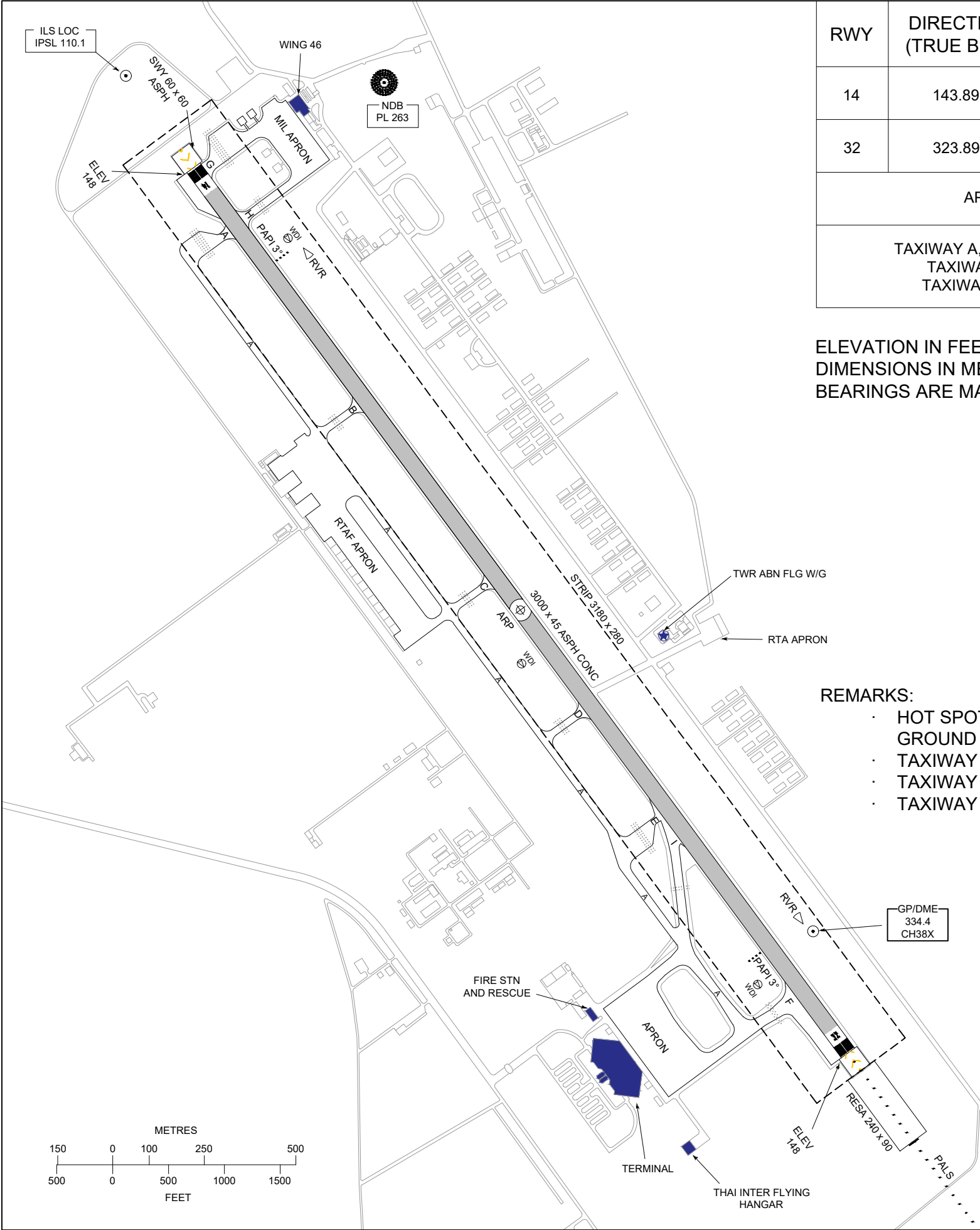
MARKING AIDS RWY 14/32 AND EXIT TWY
