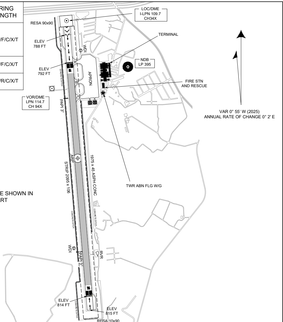
MARKING AIDS RWY 18/36 AND EXIT TWY
