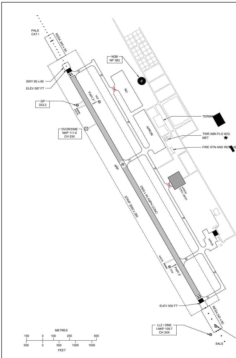
MARKING AIDS RWY 15/33 AND EXIT TWY
