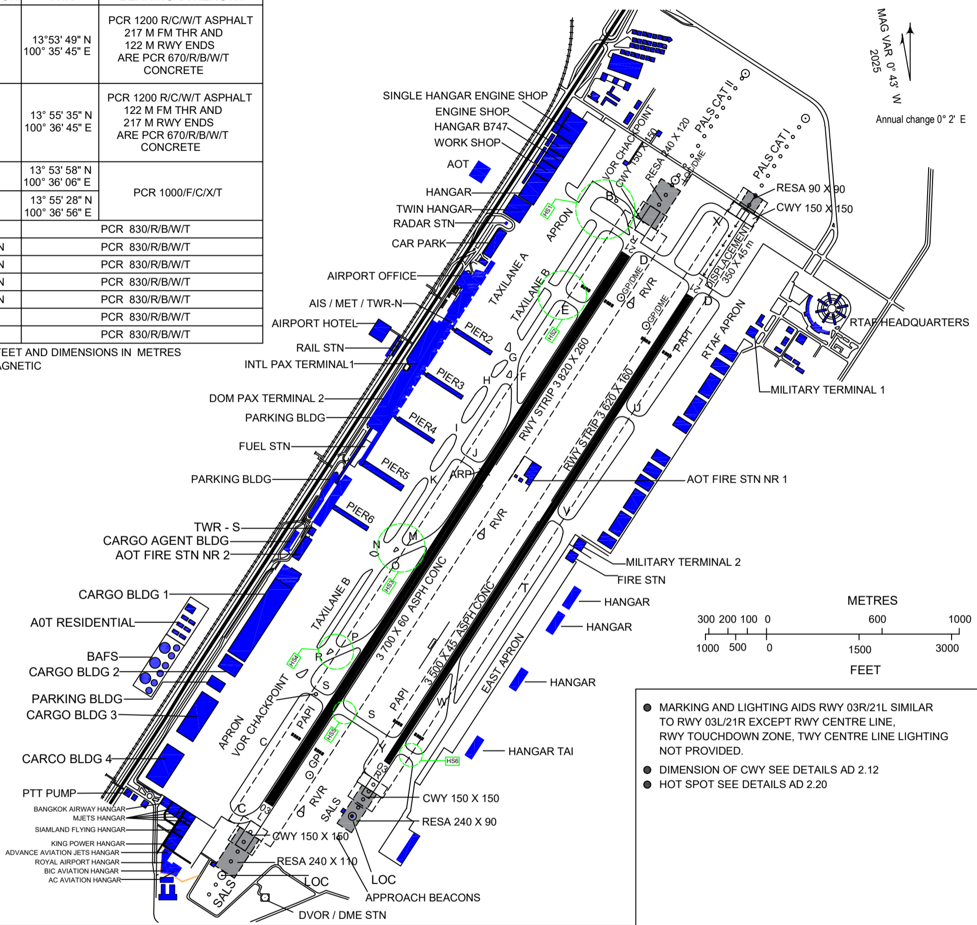
MARKING AIDS RWY 03L/21R AND EXIT TWY
