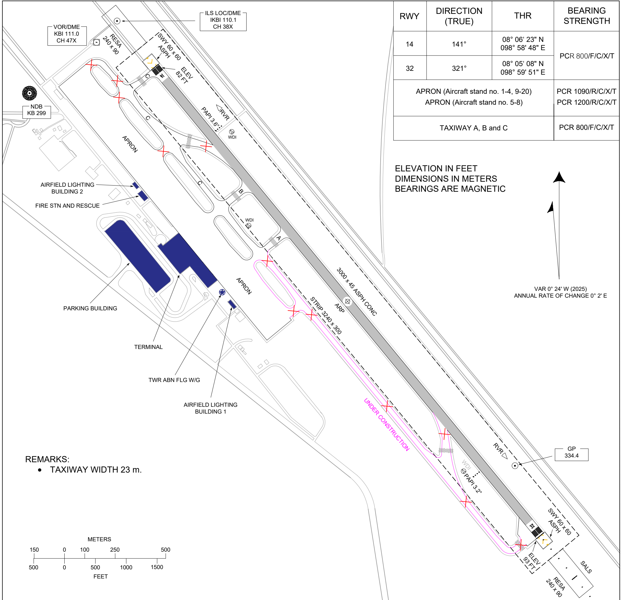
MARKING AIDS RWY 14/32 AND EXIT TWY
