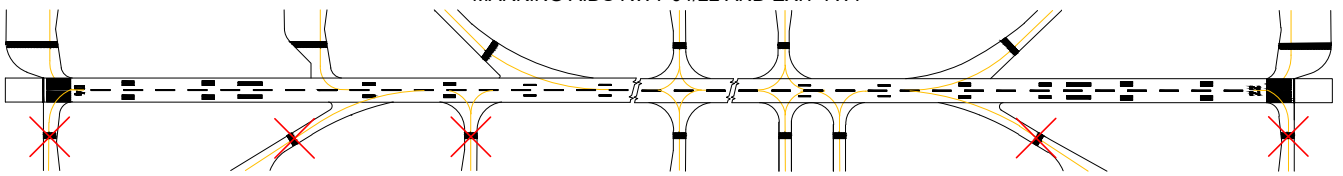
LIGHTING AIDS RWY 04/22 AND EXIT TWY
