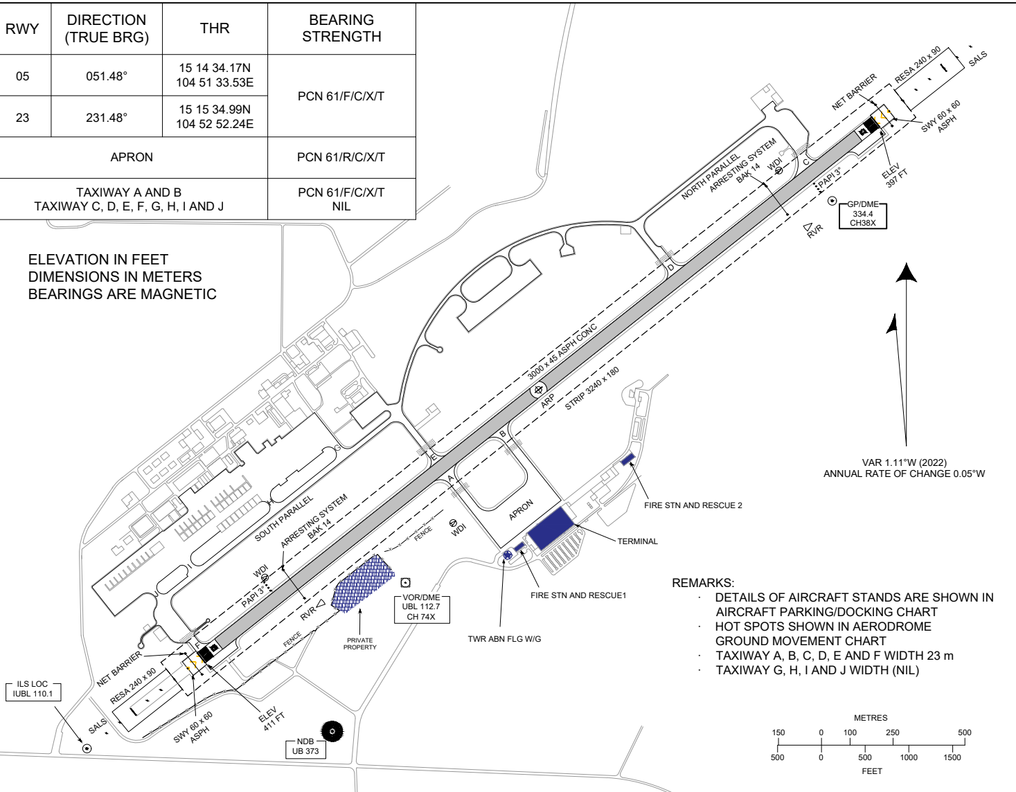
MARKING AIDS RWY 05/23 AND EXIT TWY
