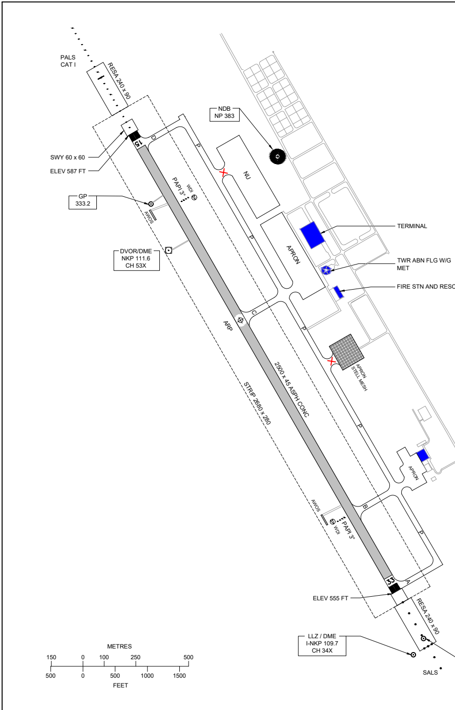
MARKING AIDS RWY 15/33 AND EXIT TWY
