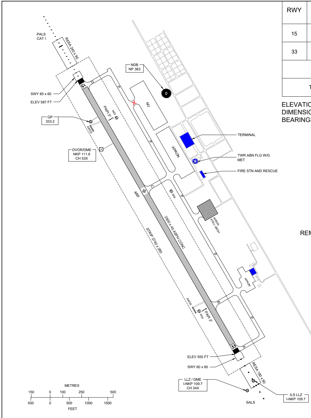
MARKING AIDS RWY 15/33 AND EXIT TWY
