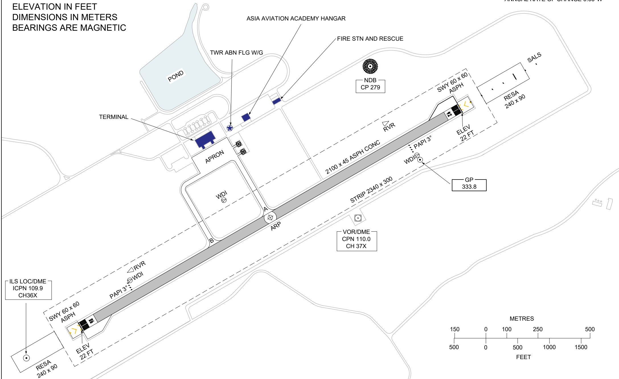
MARKING AIDS RWY 06/24 AND EXIT TWY
