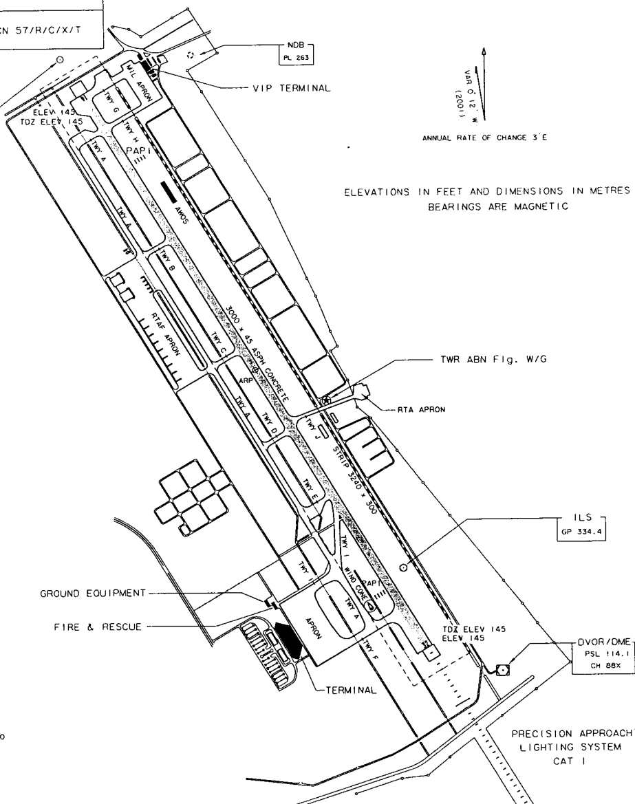
MARKING AIDS RWY 14/32 AND EXIT TWY
