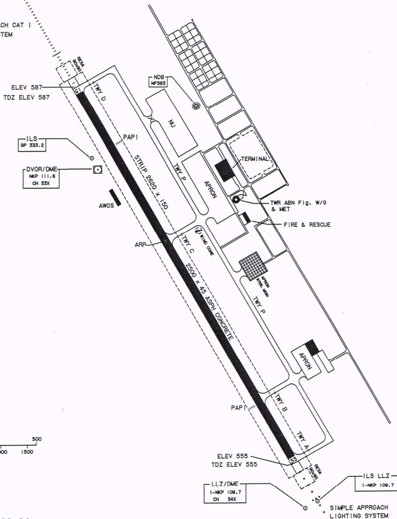
MARKING AIDS RWY 15/33 AND EXIT TWY
