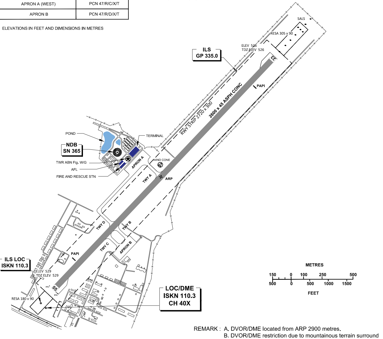
MARKING AIDS RWY 05/23 AND EXIT TWY
