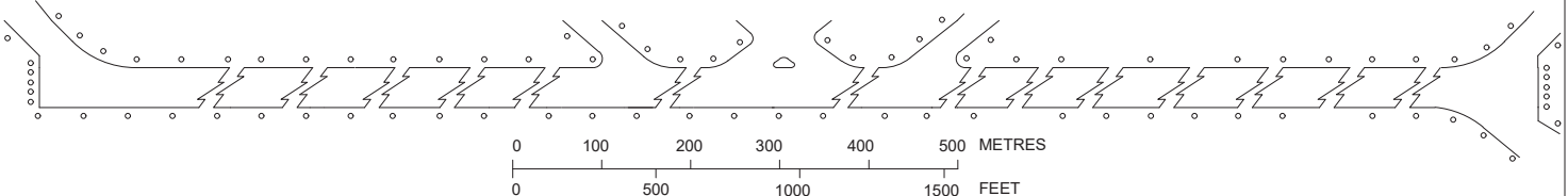
LIGHTING AIDS RWY 08/26 AND EXIT TWY
