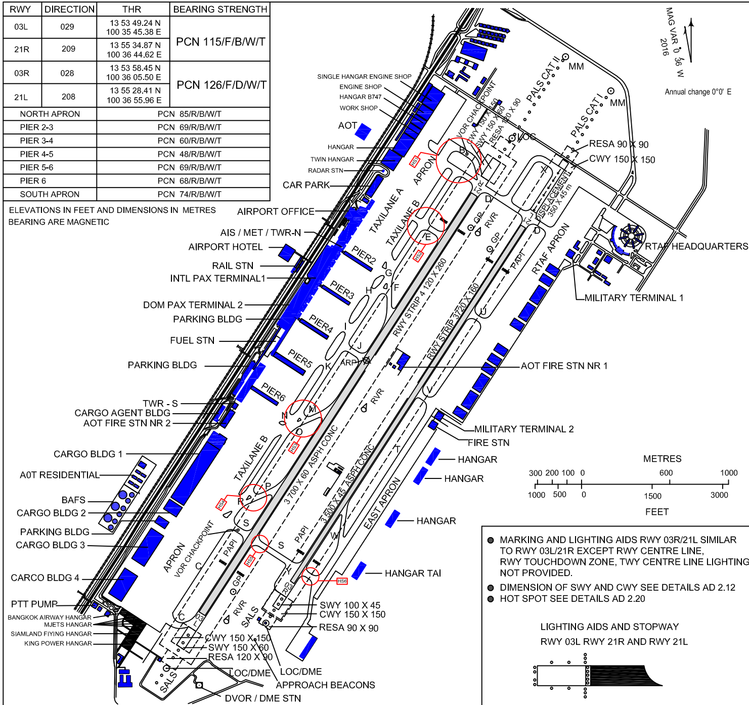
MARKING AIDS RWY 03L/21R AND EXIT TWY
