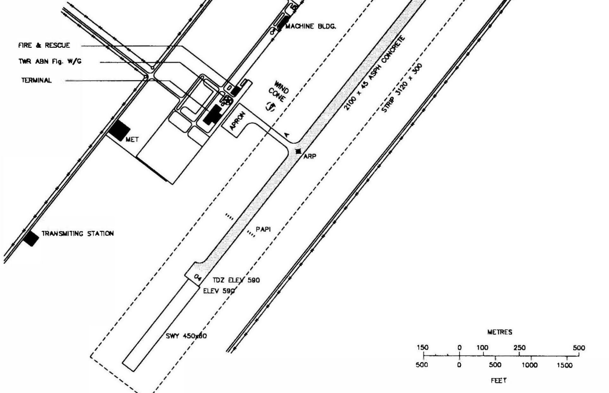
MARKING AIDS RWY 04/22 AND EXIT TWY
