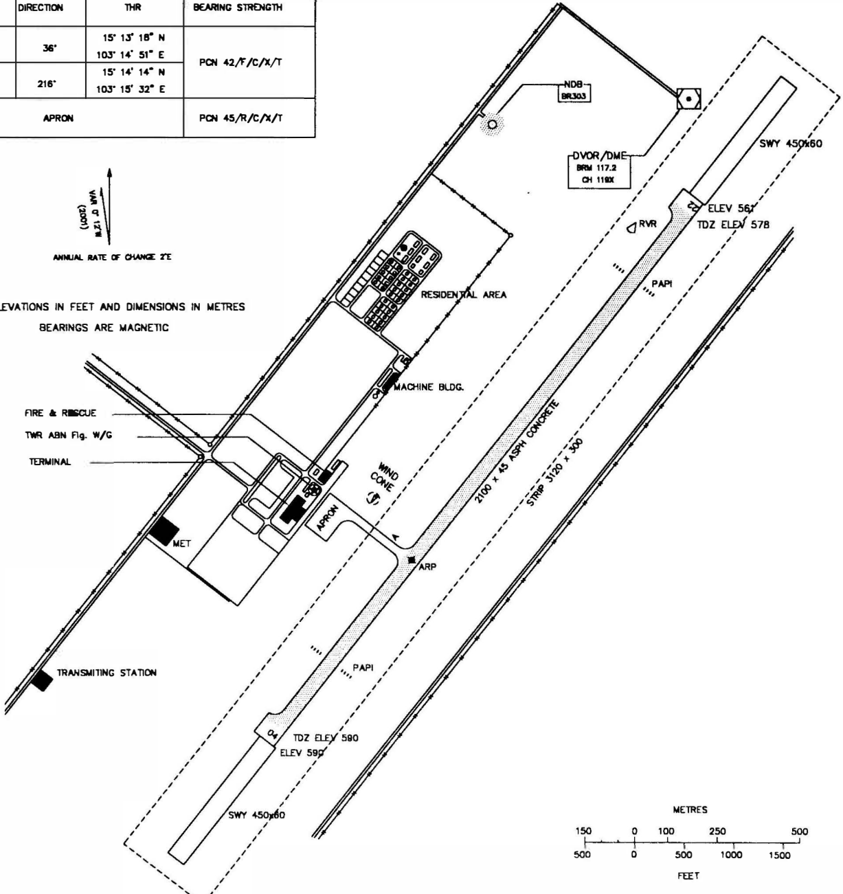
MARKING AIDS RWY 04/22 AND EXIT TWY
