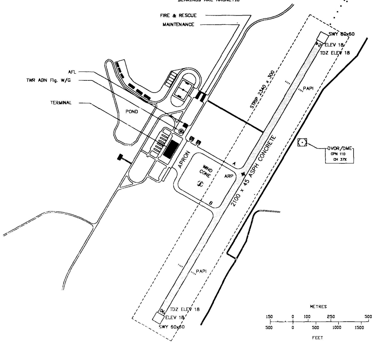
MARKING AIDS RWY 06/24 AND EXIT TWY
